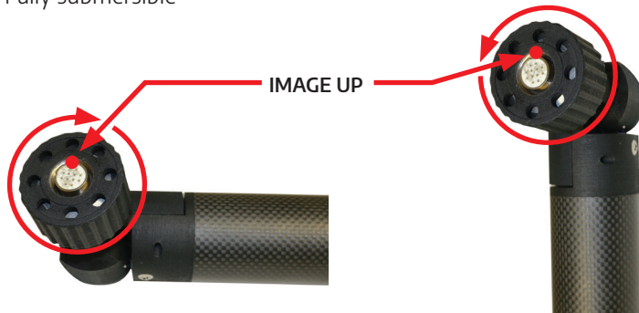
CAMERA CONNECTOR CAN BE ROTATED 90° DEPENDING UPON HORIZONTAL OR VERTICAL USE TO KEEP IMAGE UPRIGHT
